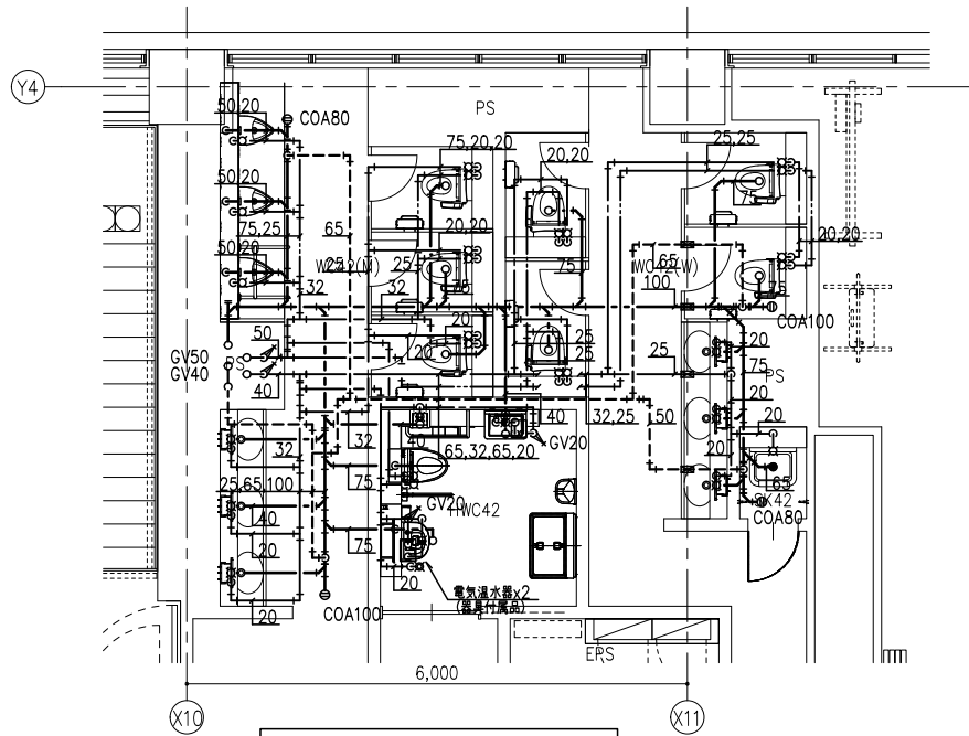
3・4階詳細図-1 S=1/50 (A1)
