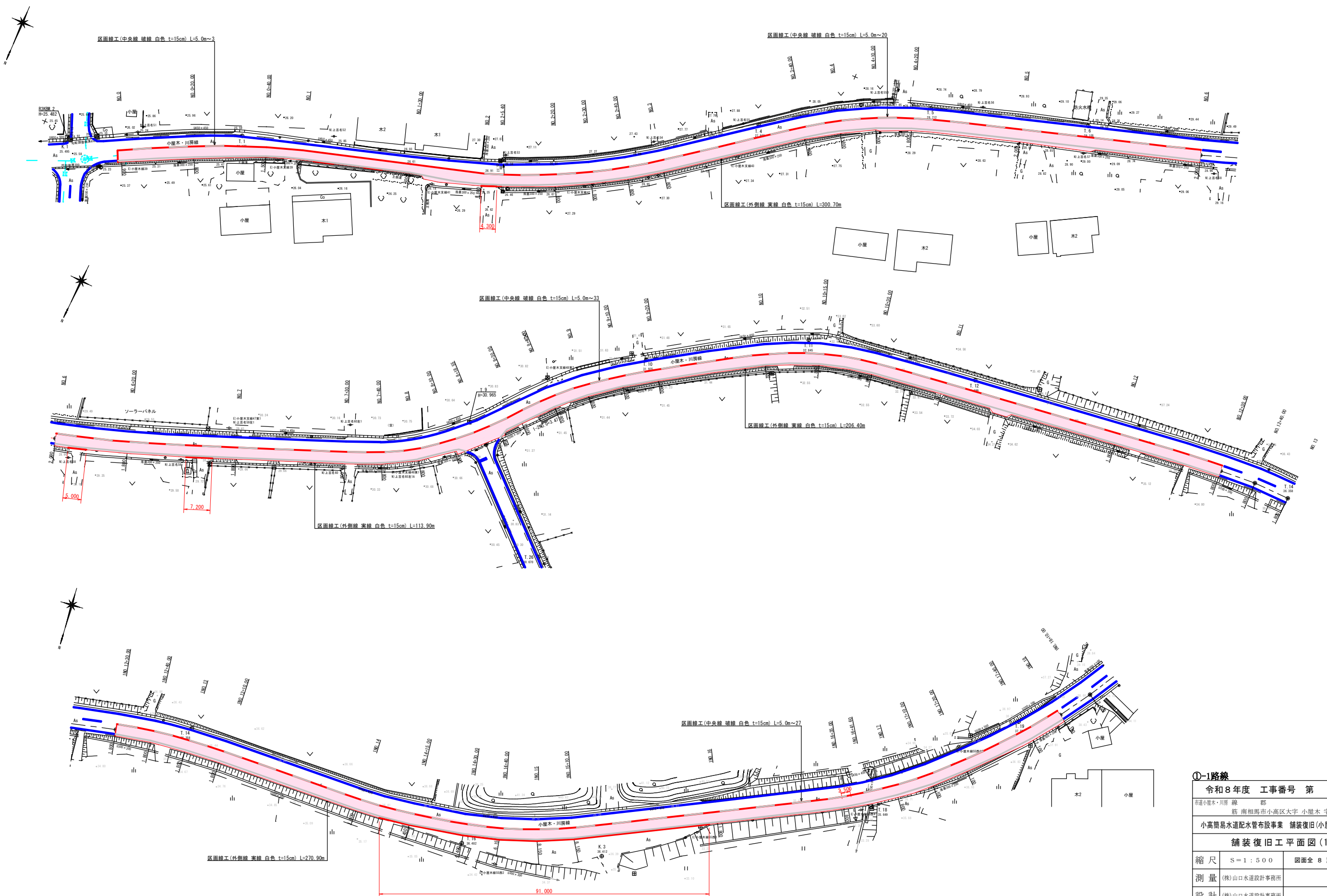
舗装復旧工平面図(1) S=1:500
